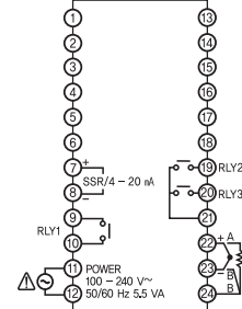
Connection diagram
