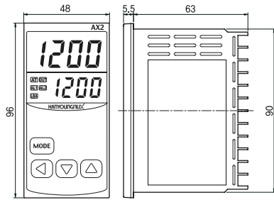
Dimension
