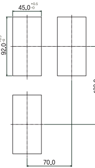
Panel cutout
